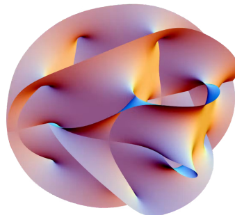
Figure 7: Higher dimensions in string theory
