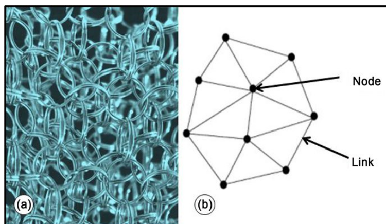
Figure 8: Spin network in loop quantum gravity
