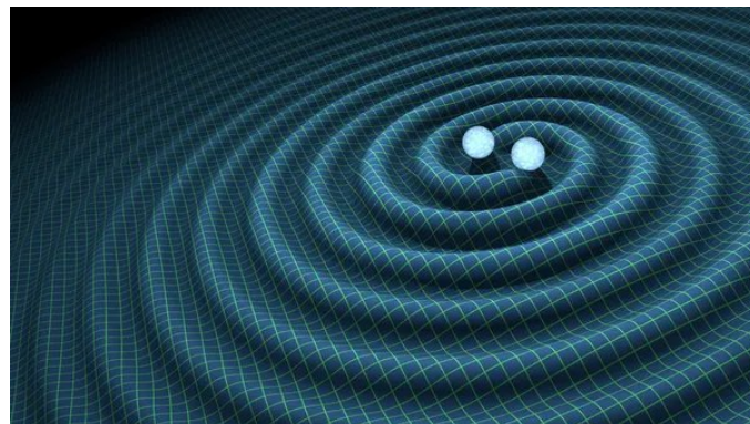
Figure 2: Gravitational waves generated by two massive objects
